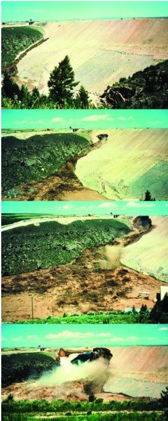
TETON DAM BREACHES — A major piping leak along the right abutment propagates headward, cutting through the crust of the dam and leading to a total breach. In the last image a tongue of “blue water” reaches through the gap. — Get Photo (/photos/teton-dam-breaches/)
